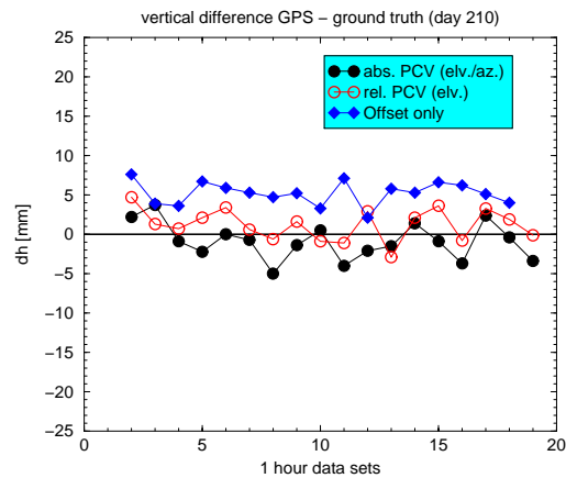
L1 - 1 hour solutions "Geodetic I" (Ref. Choke Ring)
