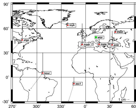
Fig. 11 - Test network, residuals +/- absolute PCV
