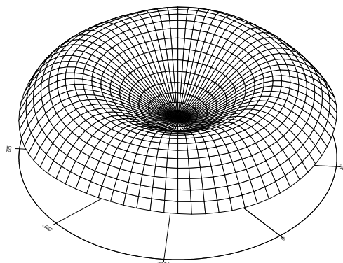
Fig. 10 - Phase pattern (qualitative) L1 Choke Ring
